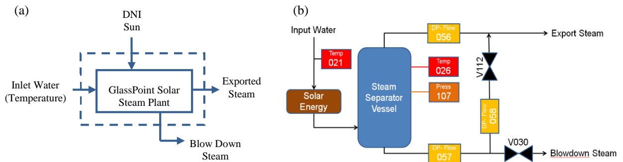
Figure 5: (a) Test boundaries, (b) Simplified schematic
