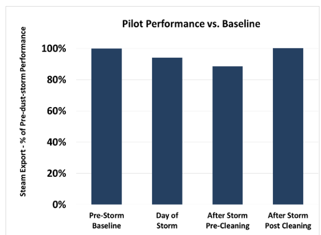
Figure 10: Performance vs. baseline, weather event
