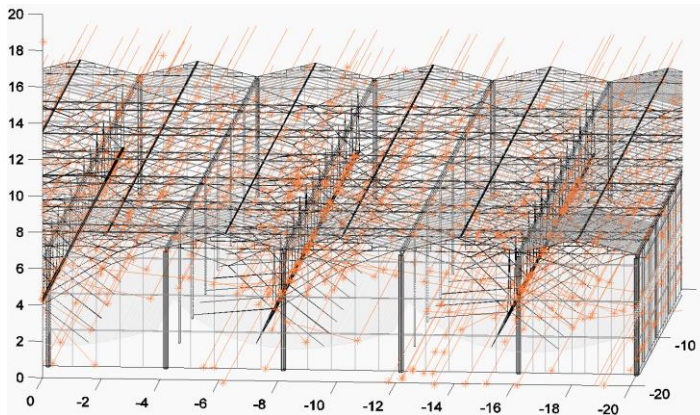
Figure 3: Ray trace diagram
