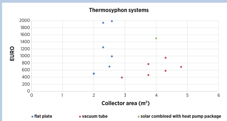
Figure 8: Comparison of final customer prices for internationally traded thermo syphon systems
